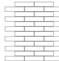
1” x 4” (25 x 106mm) Running Bond 0.94 sq. ft./sheet
